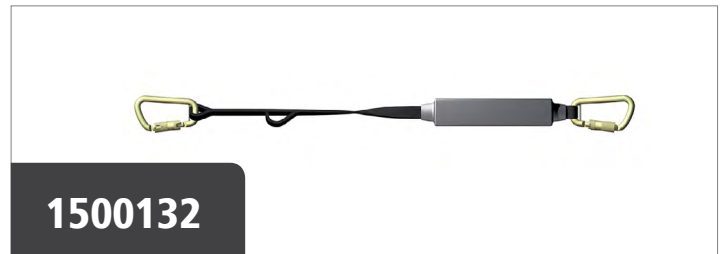
1500132 T-Pak 3 Loop Fall Arrest Lanyard 2m (3.75m Unfurled Length) Clip-back Lanyard for Fall Arrest and Work. Restraint applications. Steel autolock karabiner complete with captive pin at each end 2m in length including fittings, 1.75m of webbing unfurls during fall. Total unfurled length 3.75m long. The colour coded loops allow the user to set the lanyard to four different lengths. Alternatively the lanyard can be anchored to structural elements such as beams by passing it around and clipping back to one of the loops. Supplied with clear instructions and individually serial numbered certification. Suitable for Facilities Maintenance and Powered Access. Standard: EN 355.
