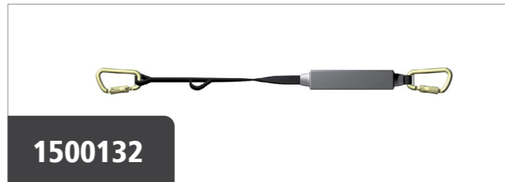
1500132 T-Pak 3 Loop Fall Arrest Lanyard 2m (3.75m Unfurled Length) Clip-back Lanyard for Fall Arrest and Work. Restraint applications. Steel autolock karabiner complete with captive pin at each end 2m in length including fittings, 1.75m of webbing unfurls during fall. Total unfurled length 3.75m long. The colour coded loops allow the user to set the lanyard to four different lengths. Alternatively the lanyard can be anchored to structural elements such as beams by passing it around and clipping back to one of the loops. Supplied with clear instructions and individually serial numbered certification. Suitable for Facilities Maintenance and Powered Access. Standard: EN 355.
