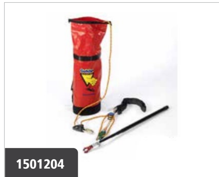
1501204 Gotcha Original Kit Suitable for Rescue from Fall Arrest Lanyards and Fall Arrest Blocks. This is a no-cut kit. The casualty is raised to release their original attachment. Rescue direction. You can raise or lower the casualty with this kit. Pre-assembled. No assembly is required by the user. Remote attachment. The casualty can be attached from a point of safety. Single person use. The Gotcha is for raising or lowering a single person. Maximum Working Length. Colour coding. The kit is colour coded for simplicity. Suitable for scaffolding and oil and gas.
